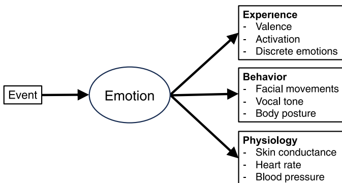
Fig. 1 Schematic of the latent view of emotions with examples for indicators of experience, behavior, and physiology. Arrows represent causal direction.
